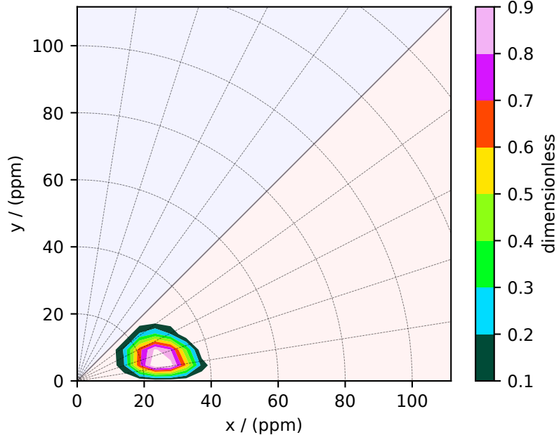
Optimum distribution
