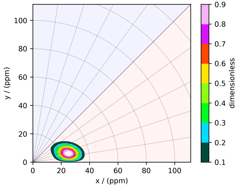
True distribution
