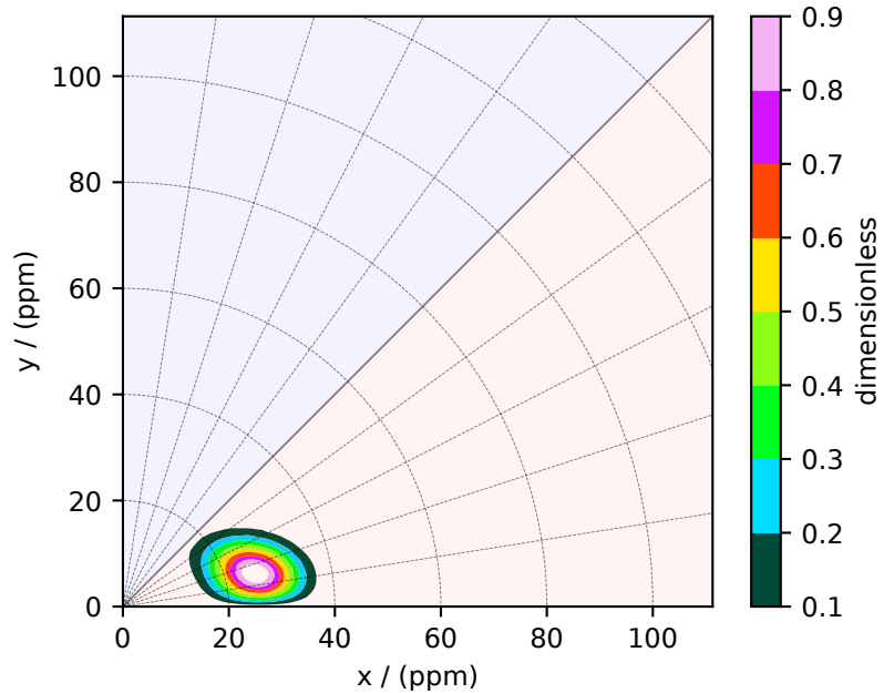
True distribution
