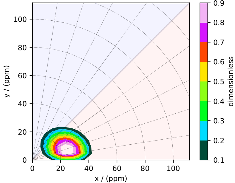
Guess distribution
