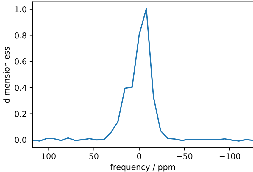
Pure anisotropic MAS spectrum
